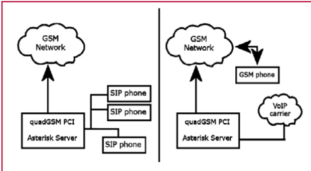
Application 1: GSM SIP gateway Application 2: GSM callback services
