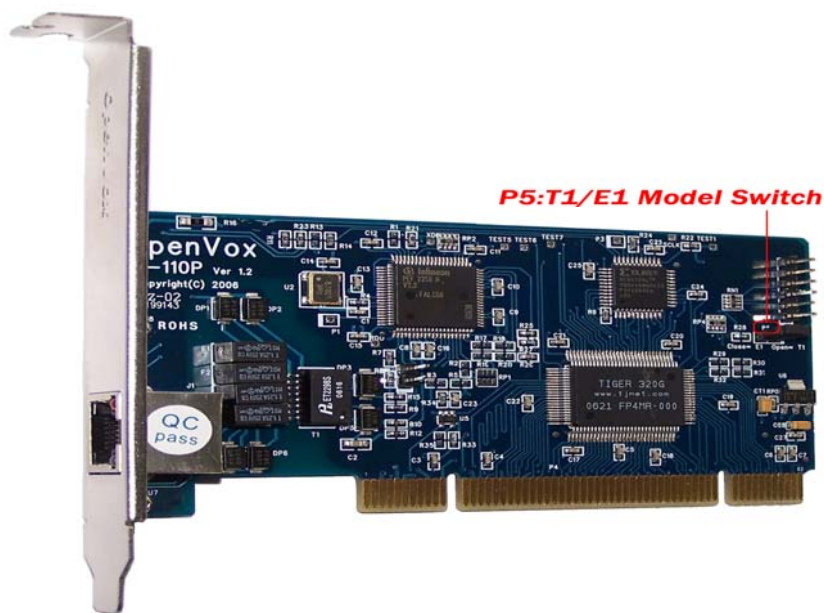
Figure 2: D110P/D110PG Hardware Configuration
