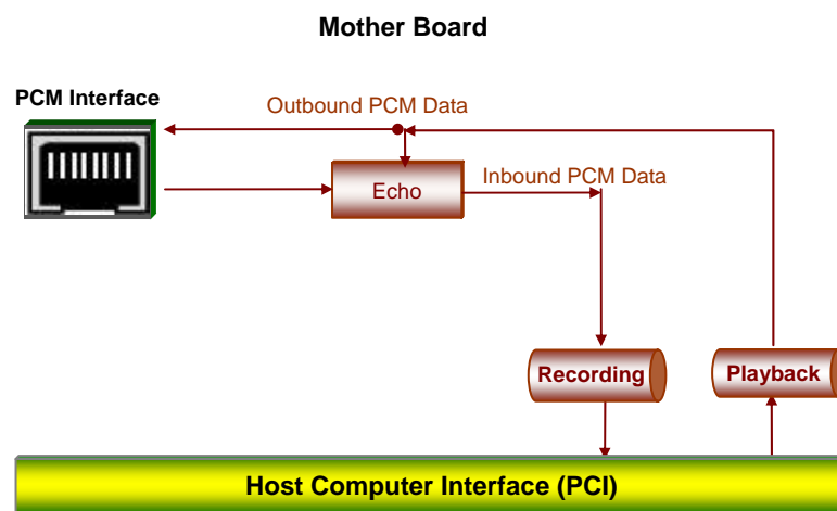
Figure 1-3 Operation Principle
