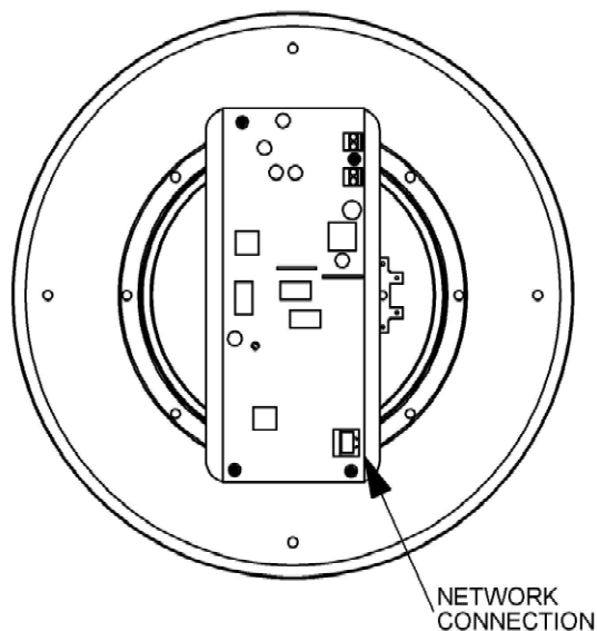
Figure 1. VIP-120-IC Connections
