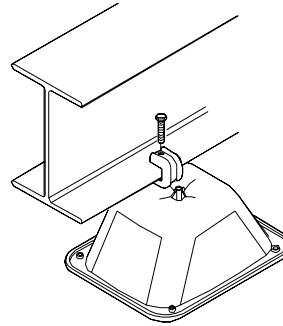
ATTACH FLEXHORN TO BEAM
